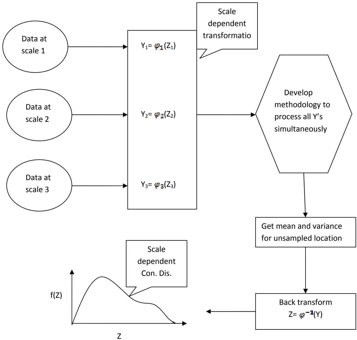
Figure 3. Mapping of point variable Z to the Gaussian variable Y
