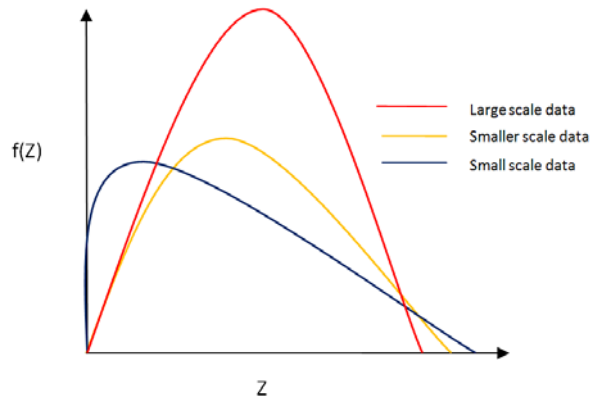
Figure 2. Hypothetical distributions for data from different scales.
